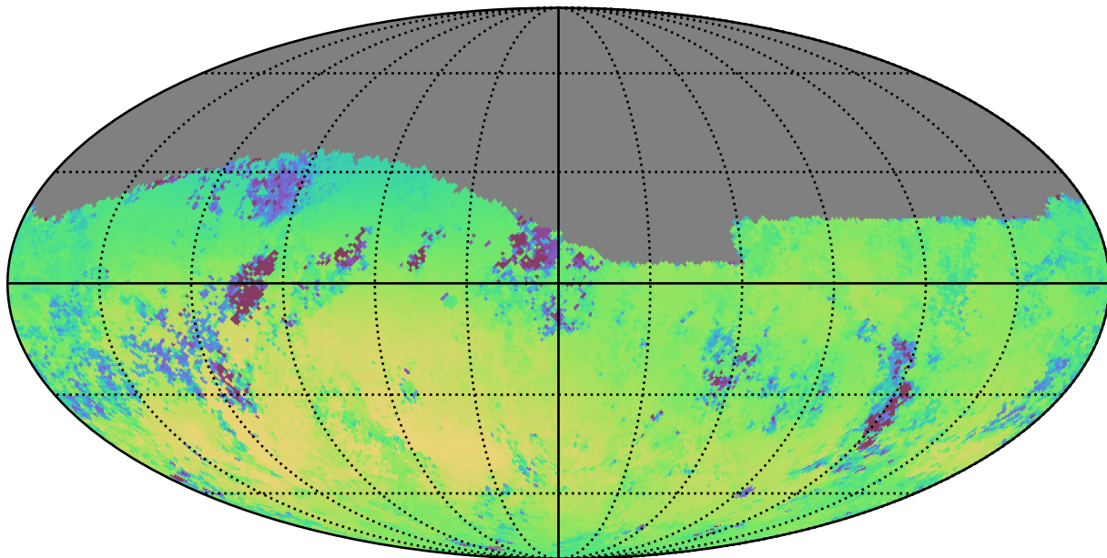
mw_roll_all_v3.3_10yrs Yr 1 r band: Median skyBrightness
