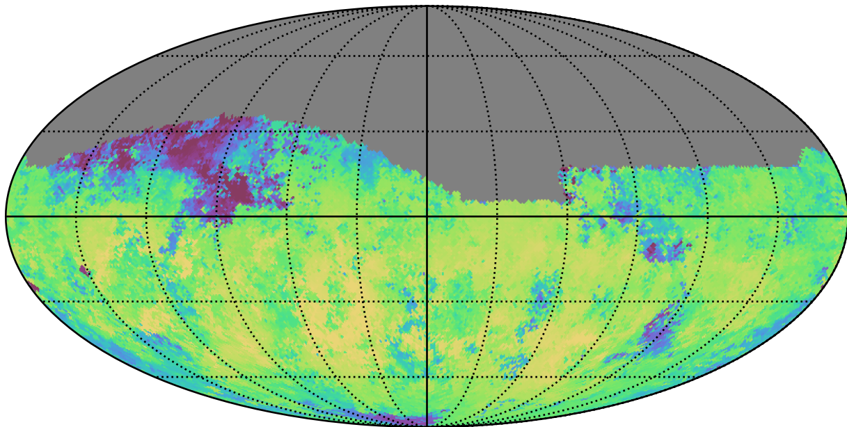
mw_roll_all_v3.3_10yrs Yr 1 i band: Median skyBrightness
