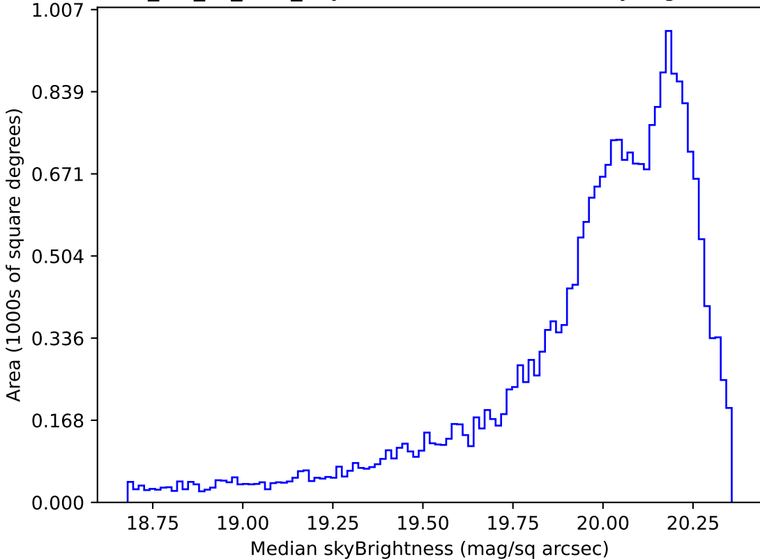
mw_roll_all_v3.3_10yrs Yr 1 i band: Median skyBrightness
