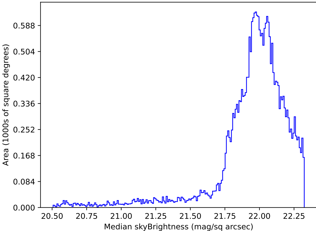
mw_roll_all_v3.3_10yrs Yr 1 g band: Median skyBrightness
