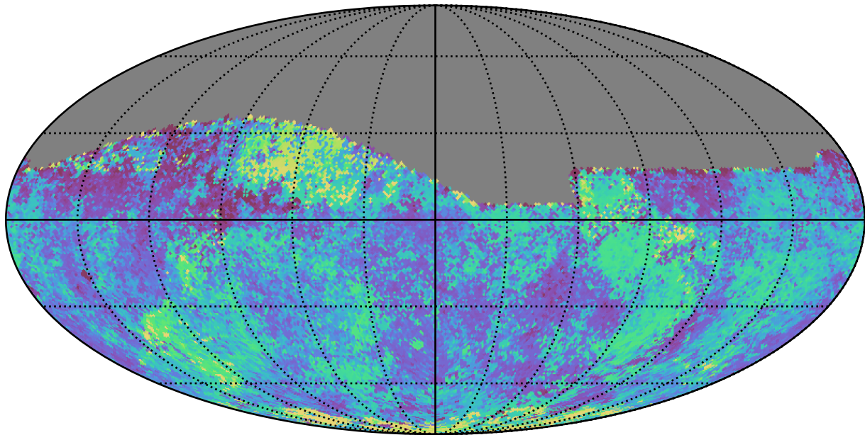
mw_roll_all_v3.3_10yrs Yr 1 all bands: Median skyBrightness
