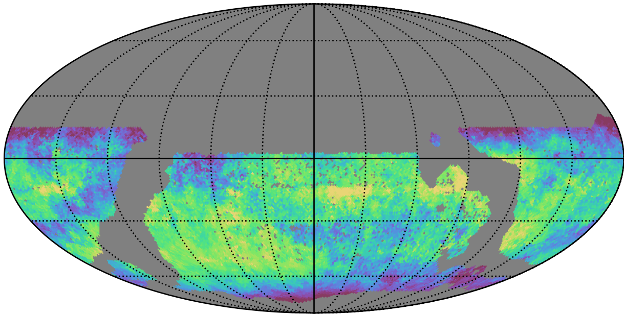
mw_roll_all_v3.3_10yrs WFD z band: Median skyBrightness
