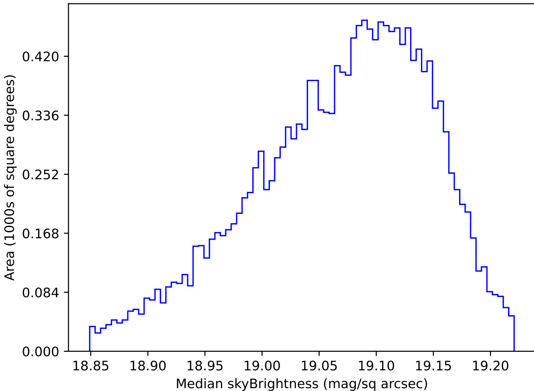
mw_roll_all_v3.3_10yrs WFD z band: Median skyBrightness
