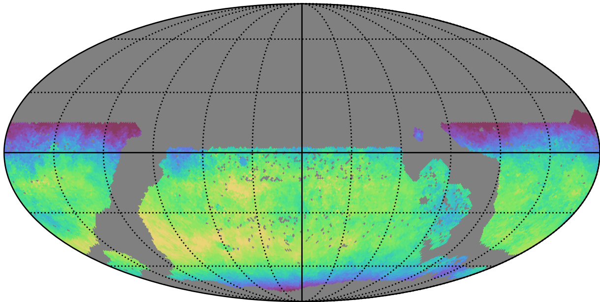
mw_roll_all_v3.3_10yrs WFD y band: Median skyBrightness
