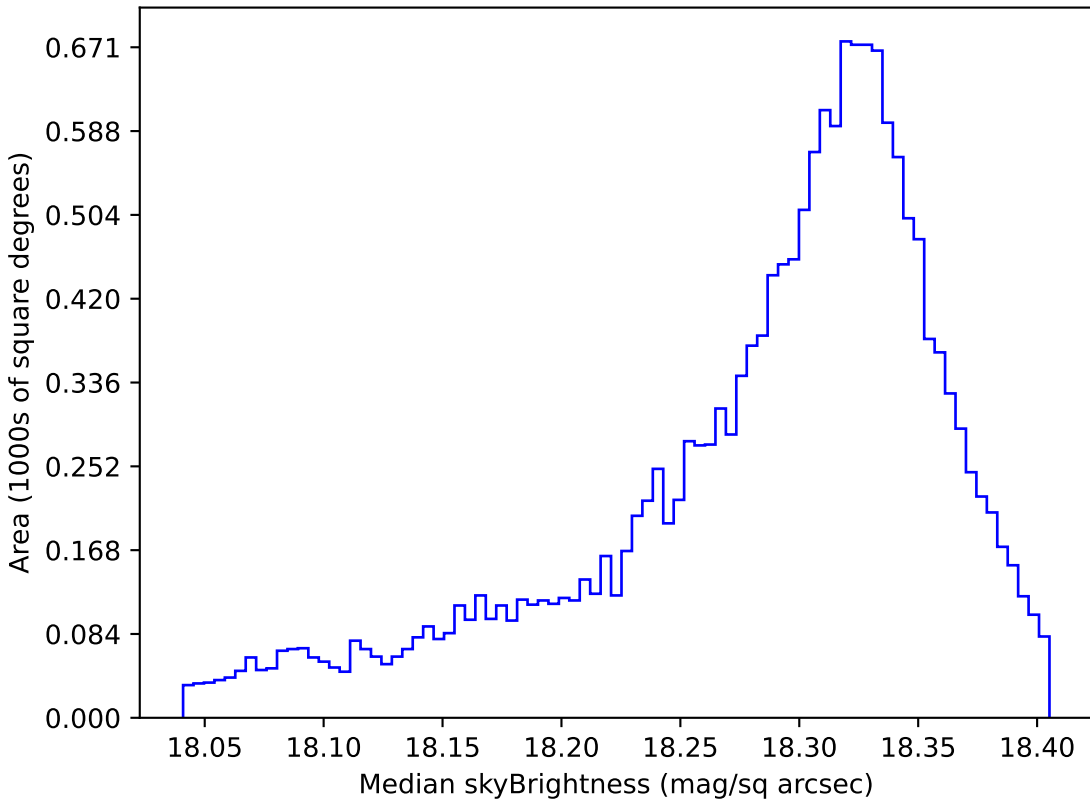
mw_roll_all_v3.3_10yrs WFD y band: Median skyBrightness
