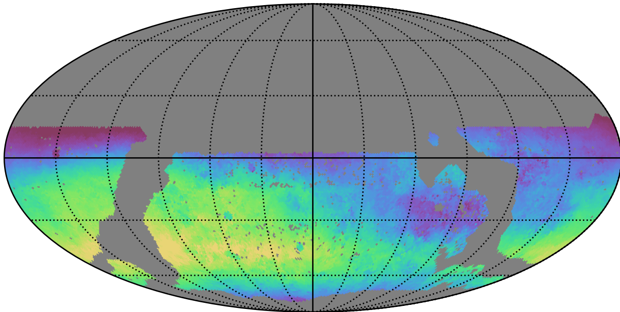
mw_roll_all_v3.3_10yrs WFD u band: Median skyBrightness
