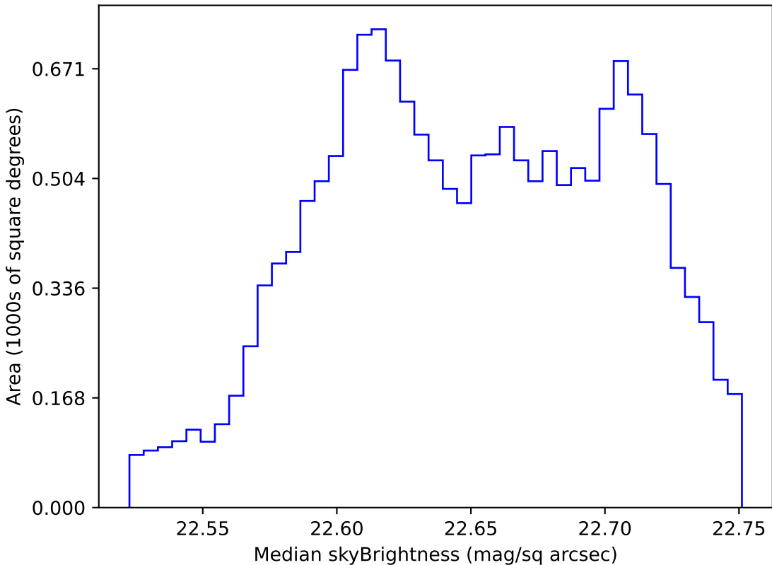
mw_roll_all_v3.3_10yrs WFD u band: Median skyBrightness
