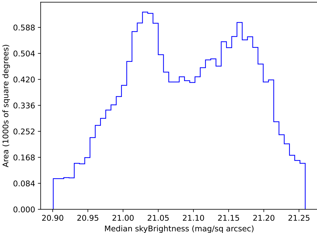
mw_roll_all_v3.3_10yrs WFD r band: Median skyBrightness
