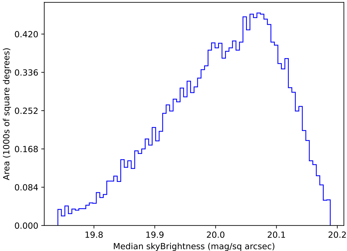
mw_roll_all_v3.3_10yrs WFD i band: Median skyBrightness
