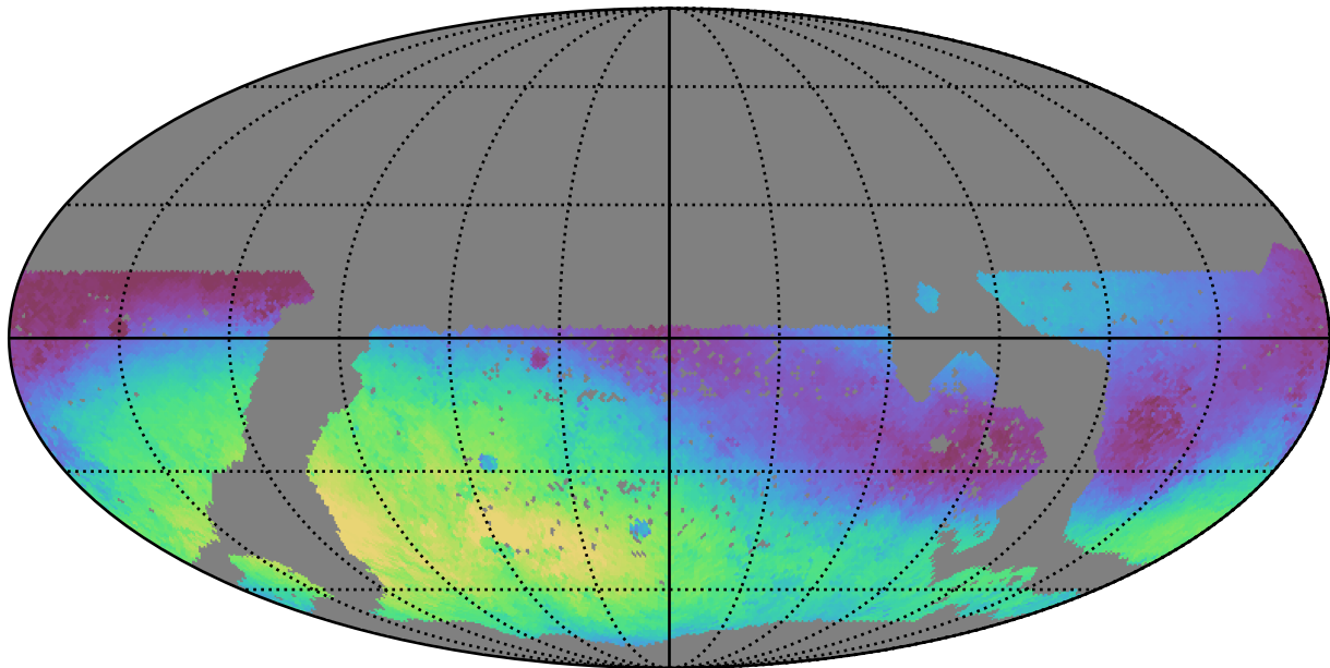
mw_roll_all_v3.3_10yrs WFD g band: Median skyBrightness
