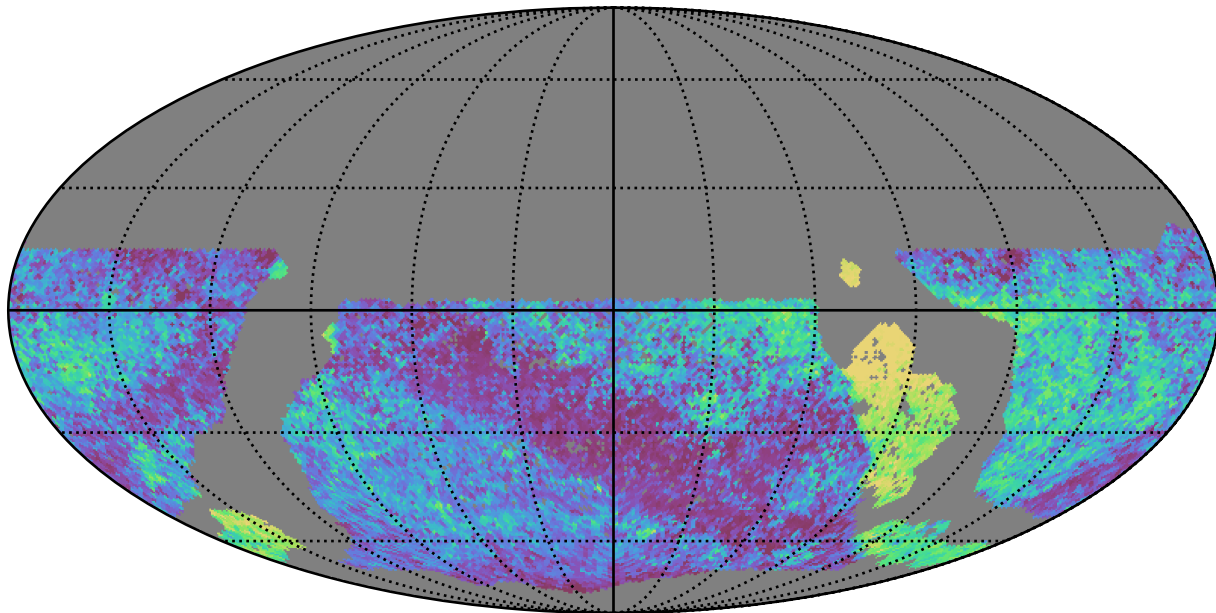
mw_roll_all_v3.3_10yrs WFD all bands: Median skyBrightness
