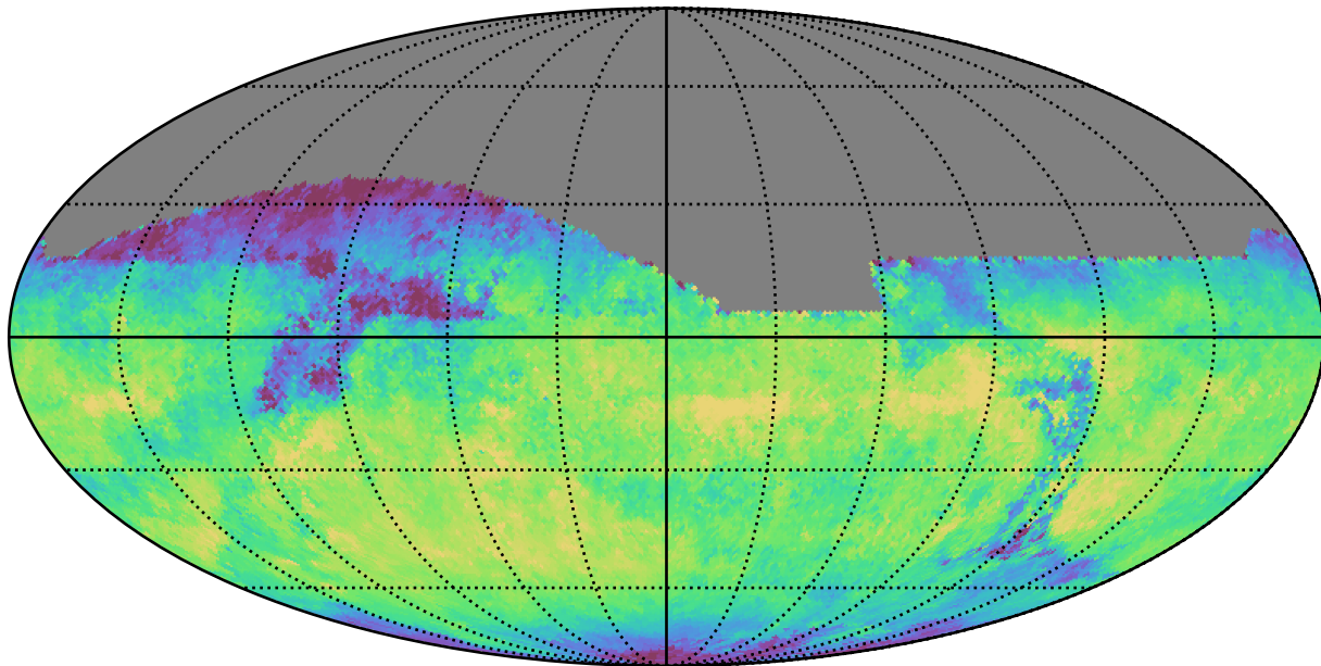
mw_roll_all_v3.3_10yrs All sky z band: Median skyBrightness
