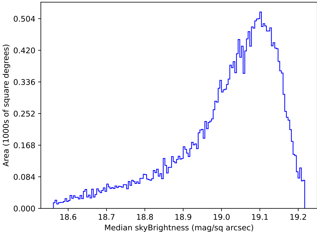
mw_roll_all_v3.3_10yrs All sky z band: Median skyBrightness
