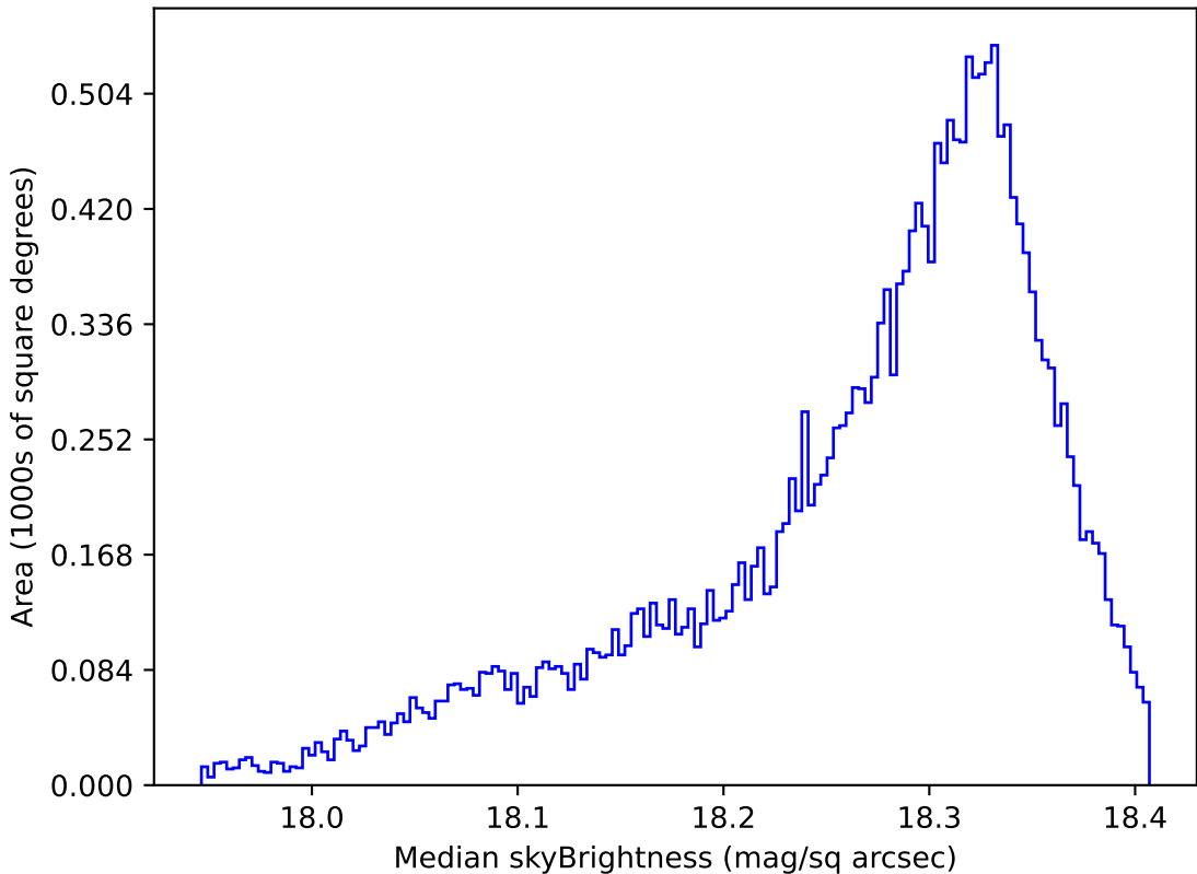
mw_roll_all_v3.3_10yrs All sky y band: Median skyBrightness
