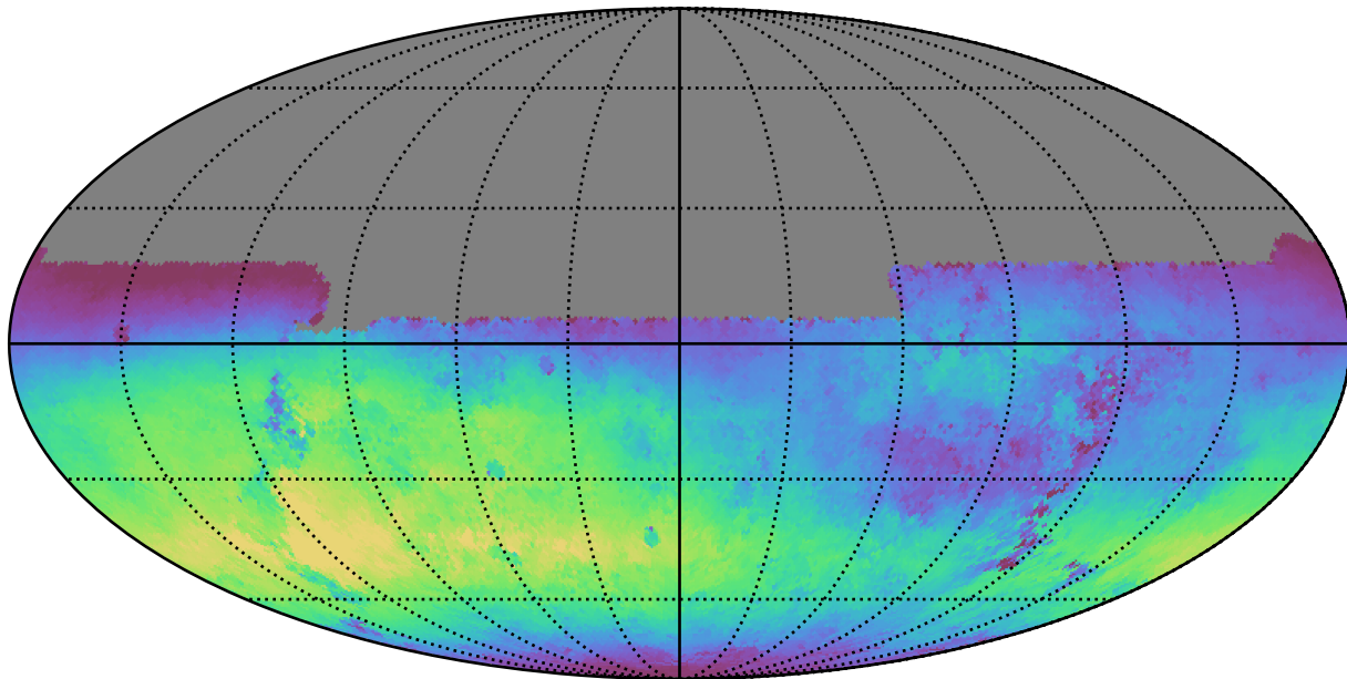
mw_roll_all_v3.3_10yrs All sky u band: Median skyBrightness
