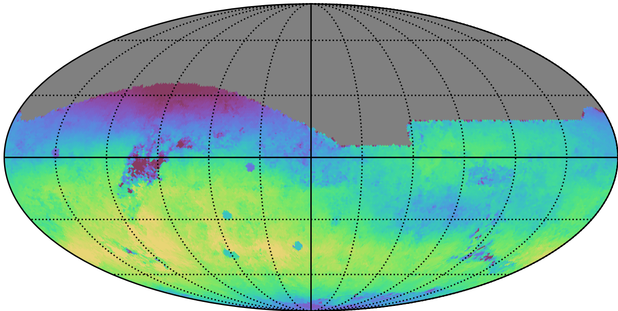
mw_roll_all_v3.3_10yrs All sky r band: Median skyBrightness
