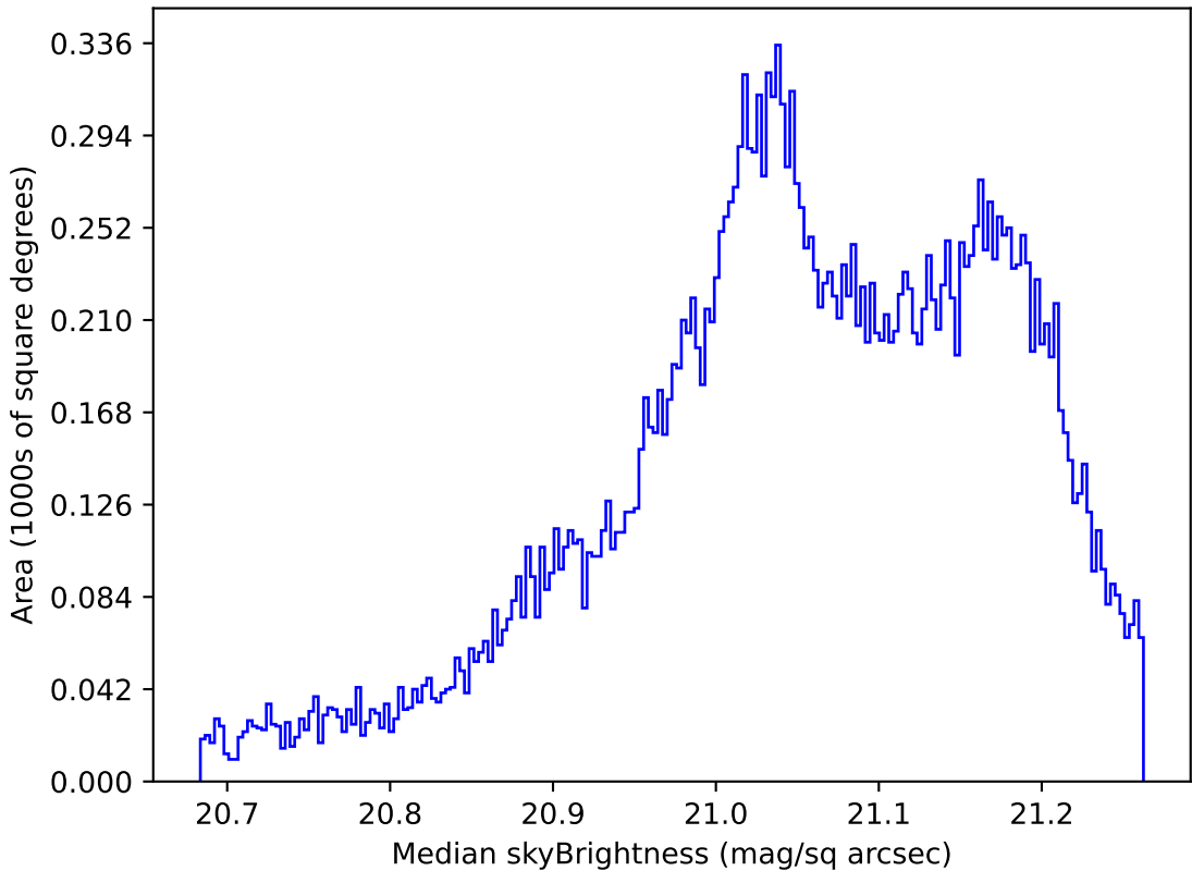
mw_roll_all_v3.3_10yrs All sky r band: Median skyBrightness
