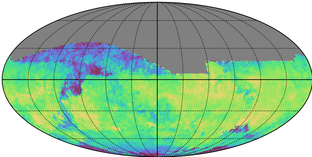
mw_roll_all_v3.3_10yrs All sky i band: Median skyBrightness
