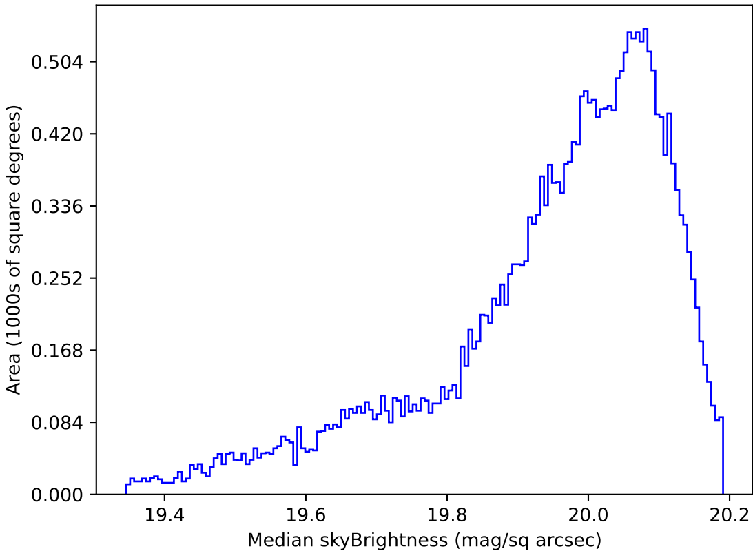
mw_roll_all_v3.3_10yrs All sky i band: Median skyBrightness
