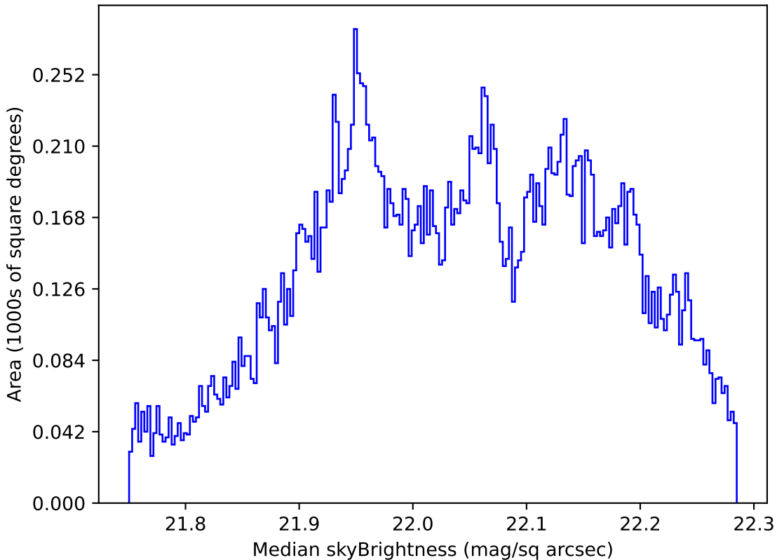
mw_roll_all_v3.3_10yrs All sky g band: Median skyBrightness
