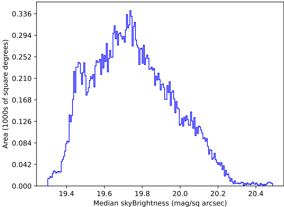
mw_roll_all_v3.3_10yrs All sky all bands: Median skyBrightness
