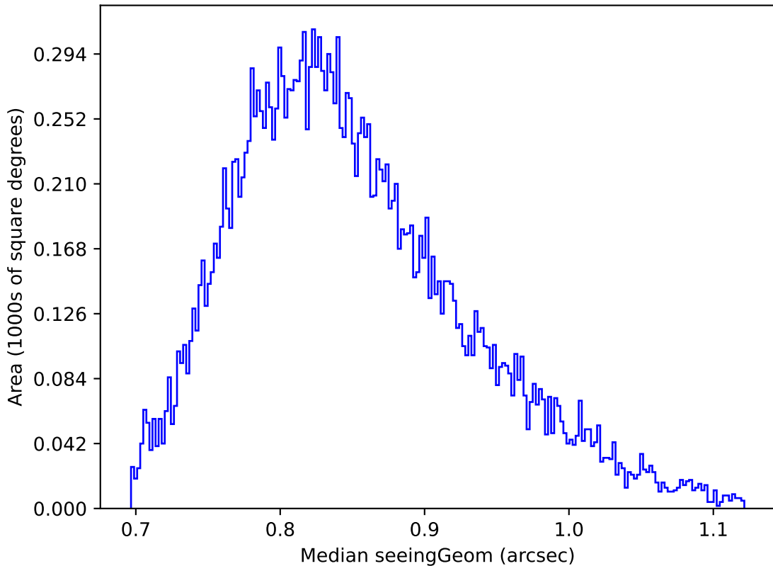
mw_roll_all_v3.3_10yrs Yr 1 y band: Median seeingGeom
