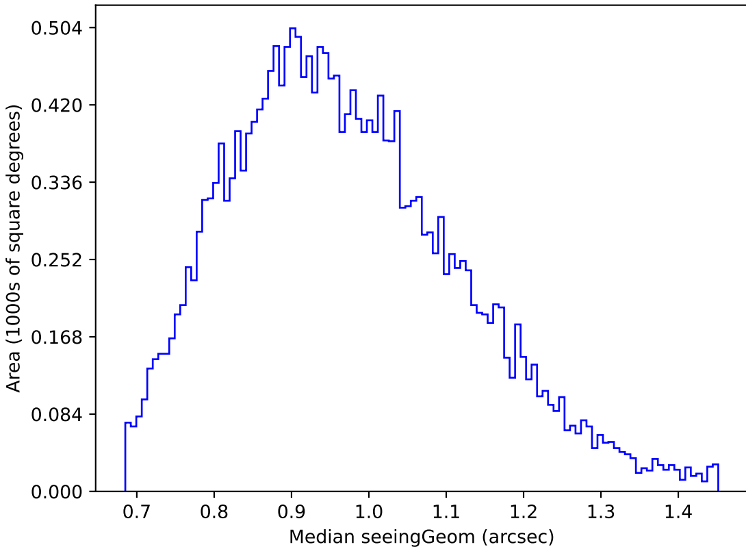
mw_roll_all_v3.3_10yrs Yr 1 u band: Median seeingGeom
