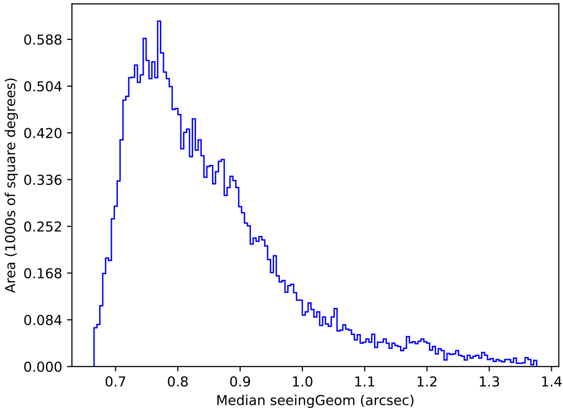
mw_roll_all_v3.3_10yrs Yr 1 r band: Median seeingGeom
