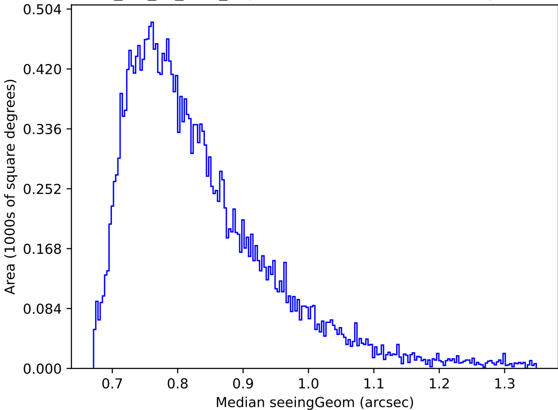
mw_roll_all_v3.3_10yrs Yr 1 i band: Median seeingGeom
