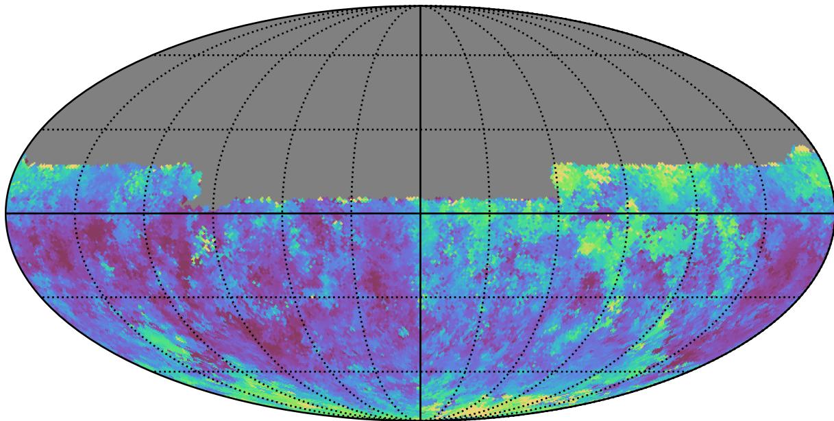
mw_roll_all_v3.3_10yrs Yr 1 y band: Median seeingEff
