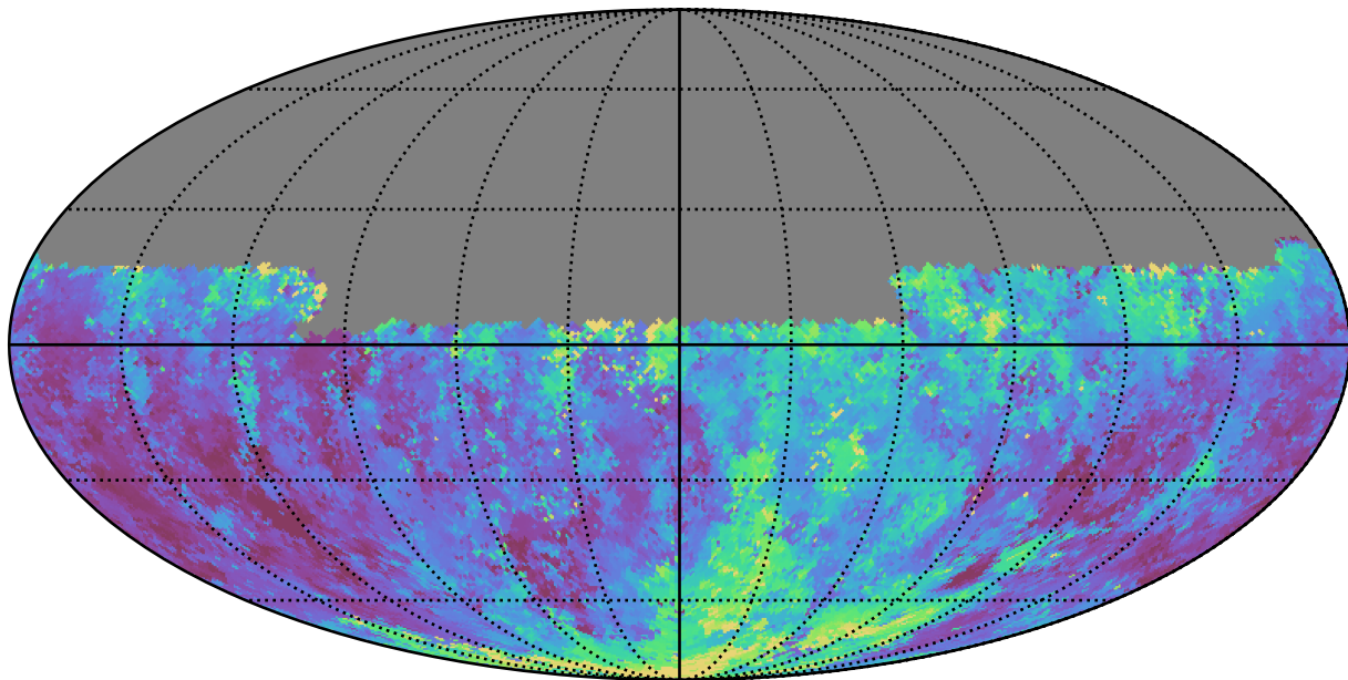
mw_roll_all_v3.3_10yrs Yr 1 u band: Median seeingEff
