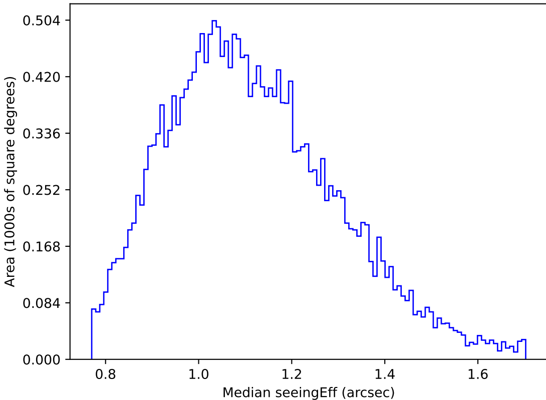
mw_roll_all_v3.3_10yrs Yr 1 u band: Median seeingEff
