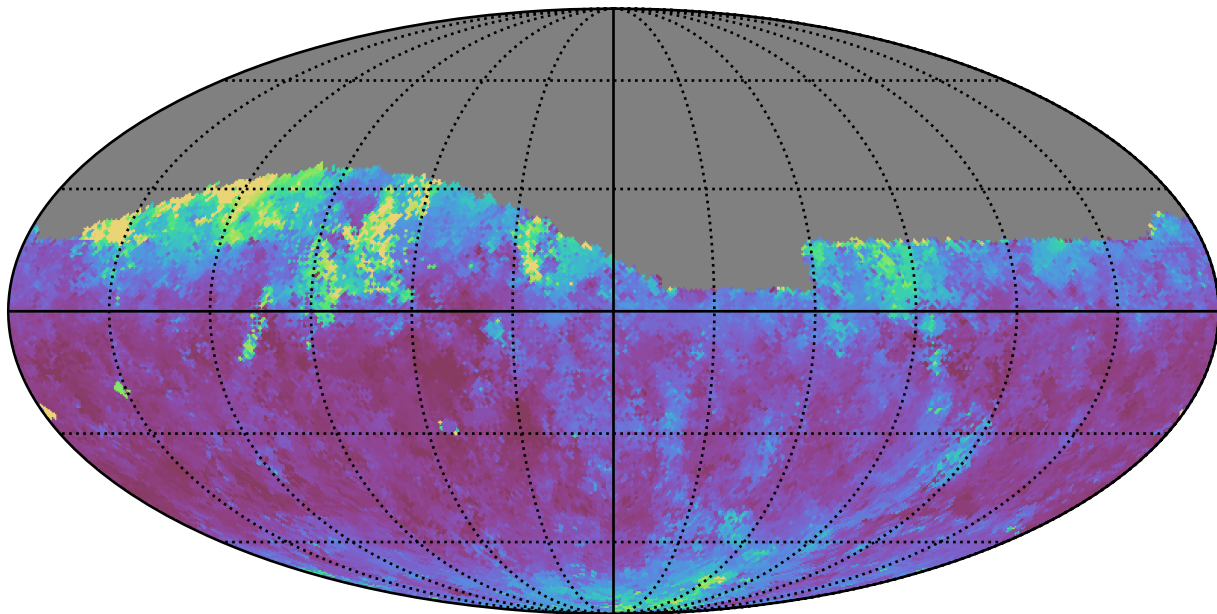
mw_roll_all_v3.3_10yrs Yr 1 i band: Median seeingEff
