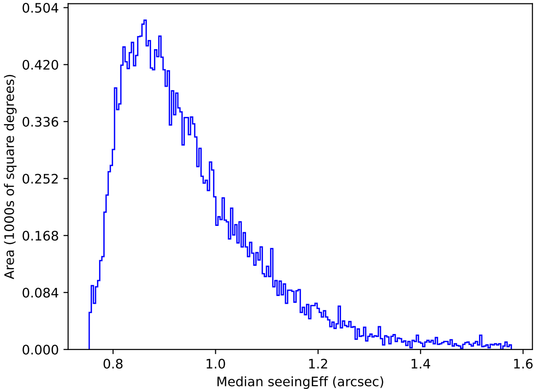
mw_roll_all_v3.3_10yrs Yr 1 i band: Median seeingEff
