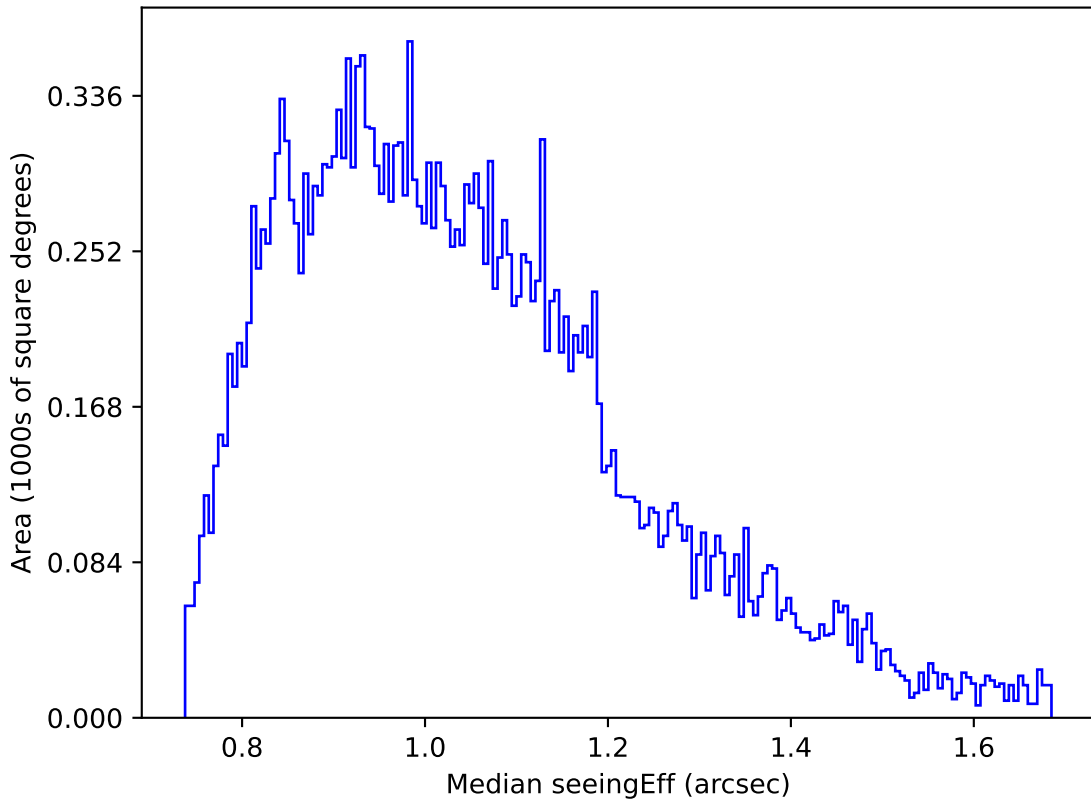
mw_roll_all_v3.3_10yrs Yr 1 g band: Median seeingEff
