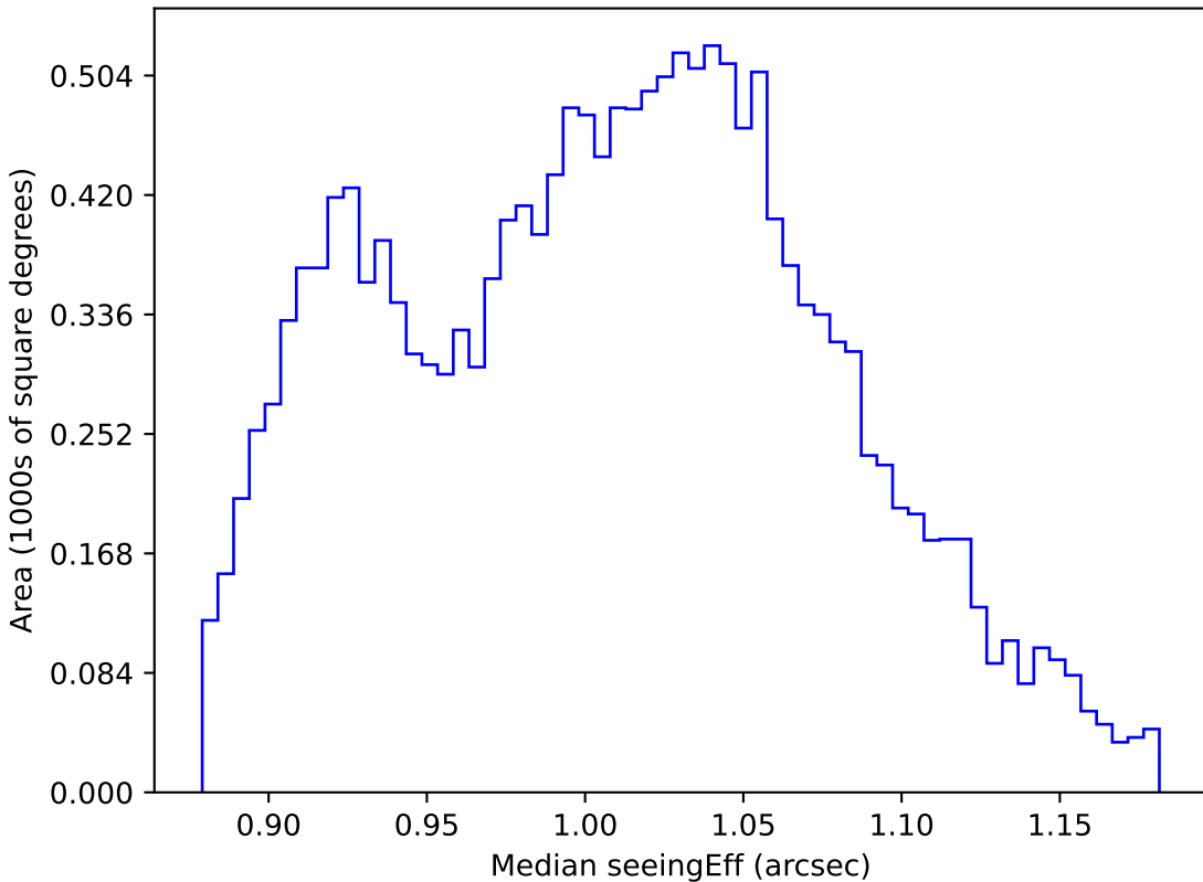
mw_roll_all_v3.3_10yrs WFD z band: Median seeingEff
