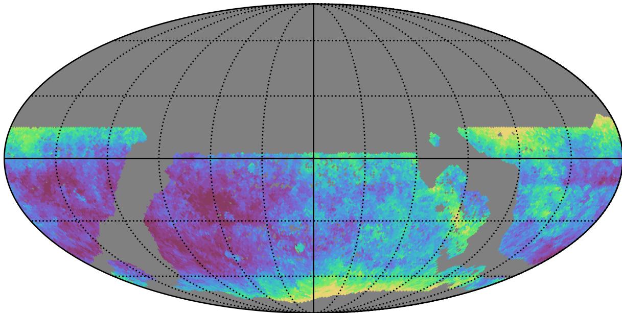
mw_roll_all_v3.3_10yrs WFD y band: Median seeingEff
