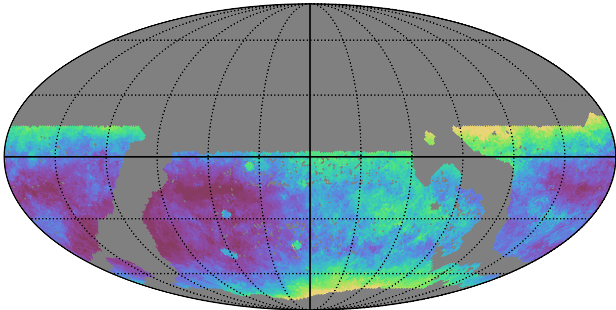
mw_roll_all_v3.3_10yrs WFD r band: Median seeingEff
