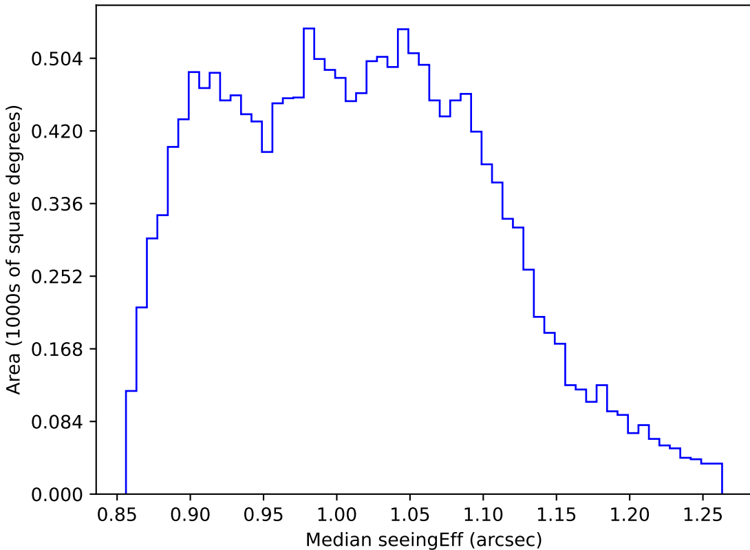
mw_roll_all_v3.3_10yrs WFD r band: Median seeingEff
