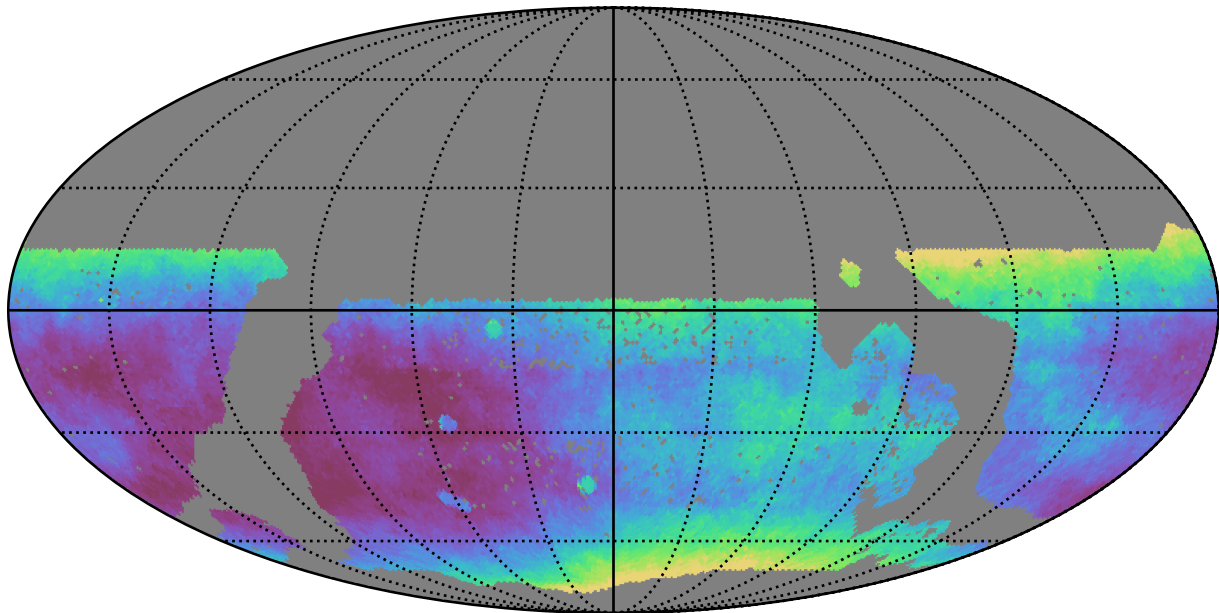
mw_roll_all_v3.3_10yrs WFD all bands: Median seeingEff
