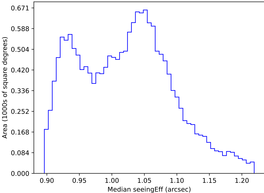
mw_roll_all_v3.3_10yrs WFD all bands: Median seeingEff
