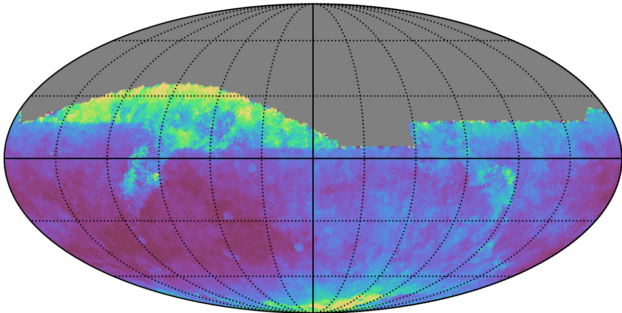
mw_roll_all_v3.3_10yrs All sky z band: Median seeingEff
