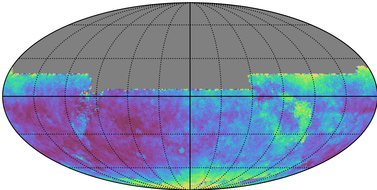
mw_roll_all_v3.3_10yrs All sky y band: Median seeingEff
