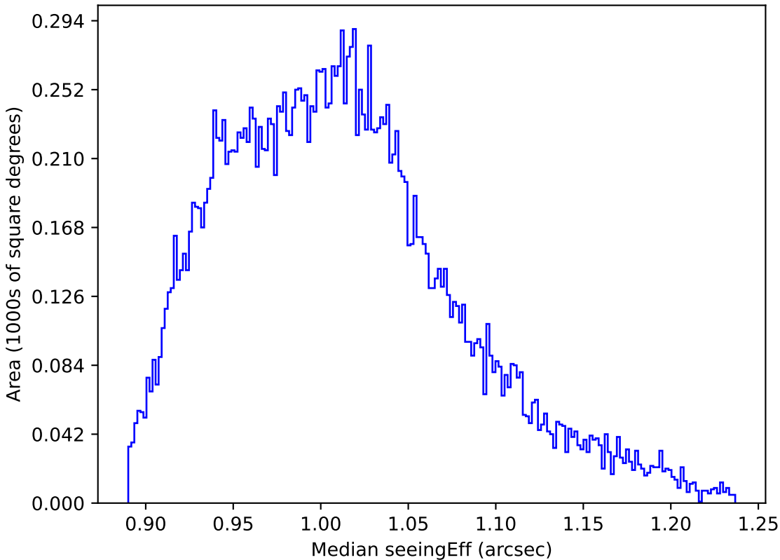
mw_roll_all_v3.3_10yrs All sky y band: Median seeingEff
