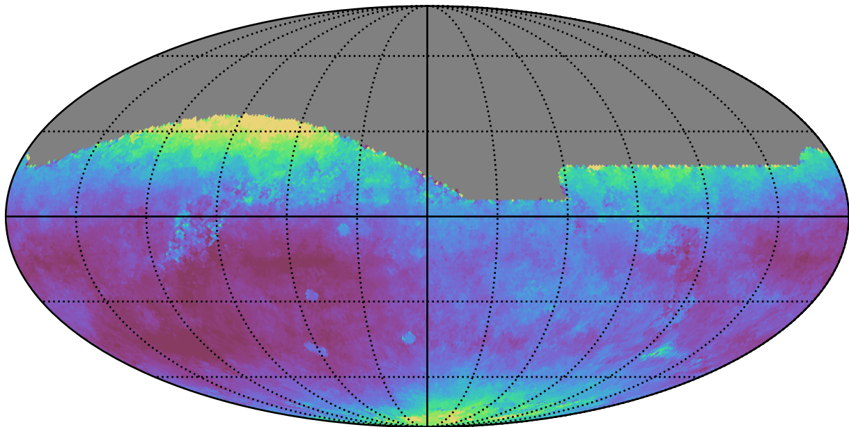
mw_roll_all_v3.3_10yrs All sky r band: Median seeingEff
