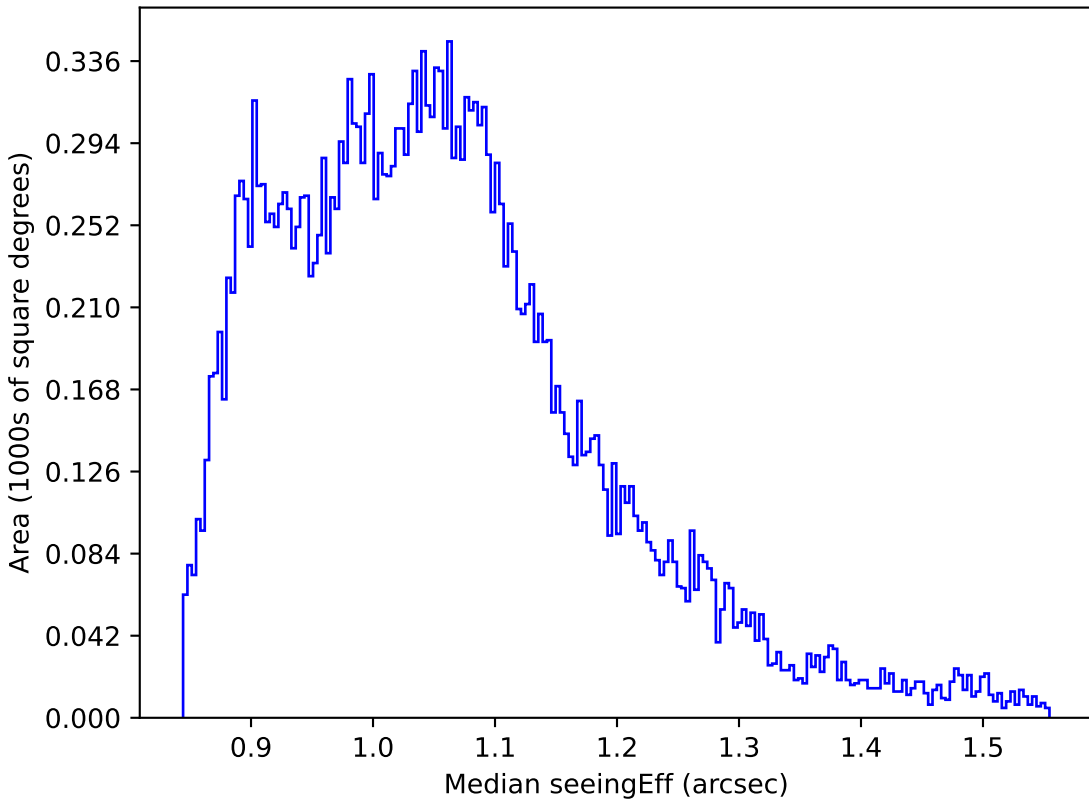
mw_roll_all_v3.3_10yrs All sky r band: Median seeingEff
