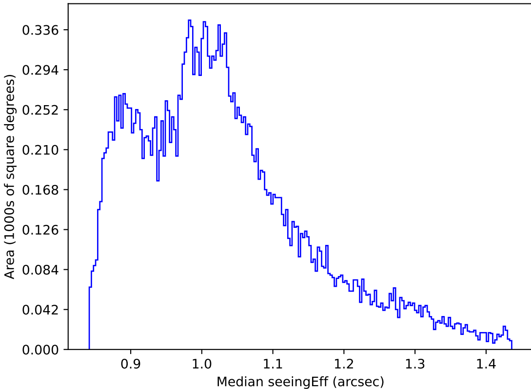
mw_roll_all_v3.3_10yrs All sky i band: Median seeingEff
