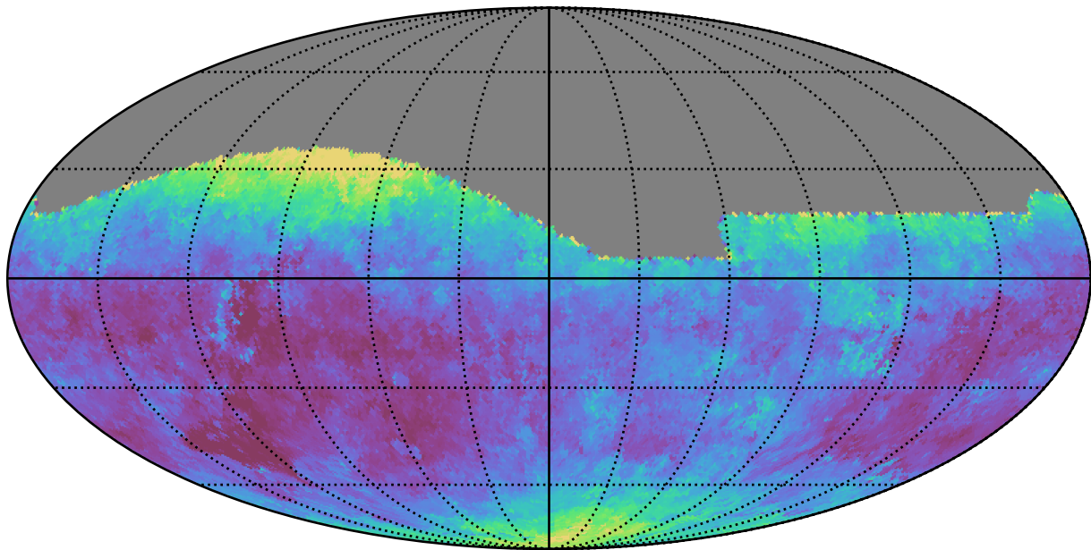
mw_roll_all_v3.3_10yrs All sky g band: Median seeingEff
