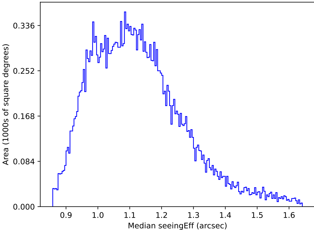
mw_roll_all_v3.3_10yrs All sky g band: Median seeingEff
