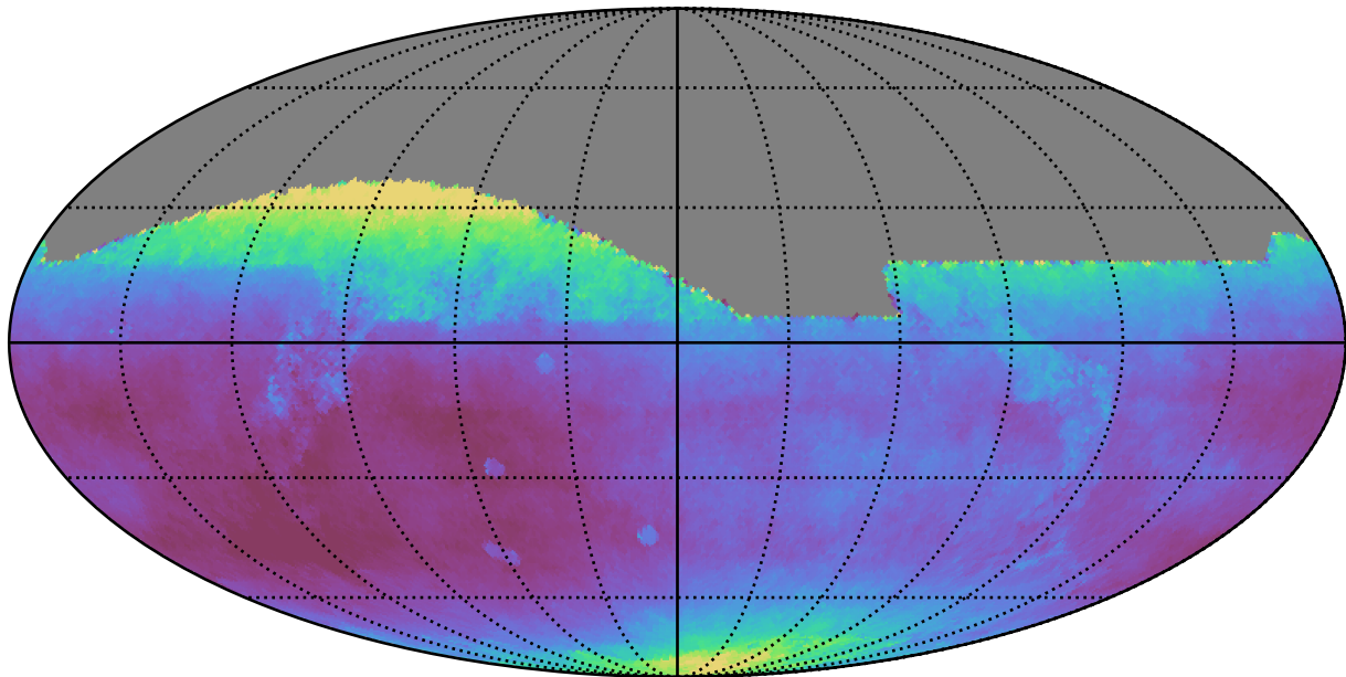
mw_roll_all_v3.3_10yrs All sky all bands: Median seeingEff
